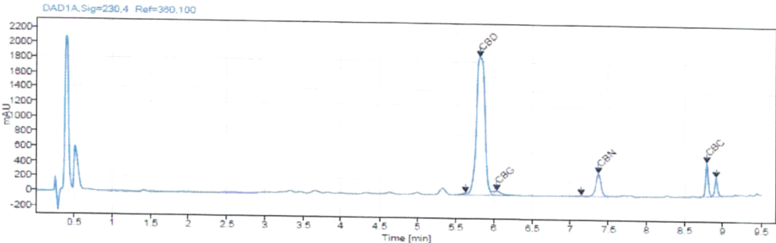
Chromatogram
